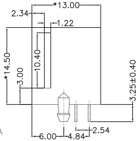
CUTAWAY VIEW
